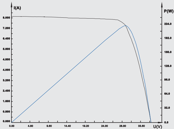
Current, Power vs. Voltage Characteristics
